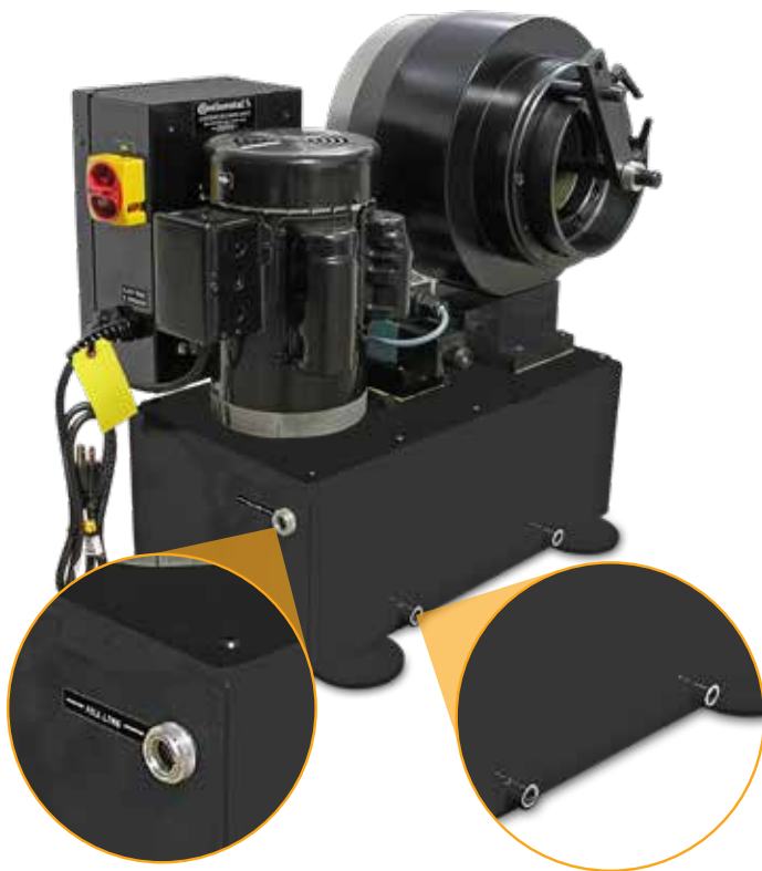
Manual back stop speeds multiple crimps of the same hose and fitting
